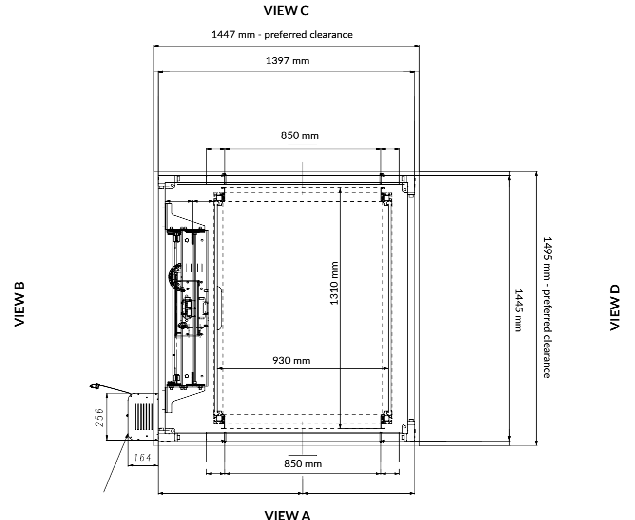
Electronics cabinet H = 1980 mm on the bottom floor
