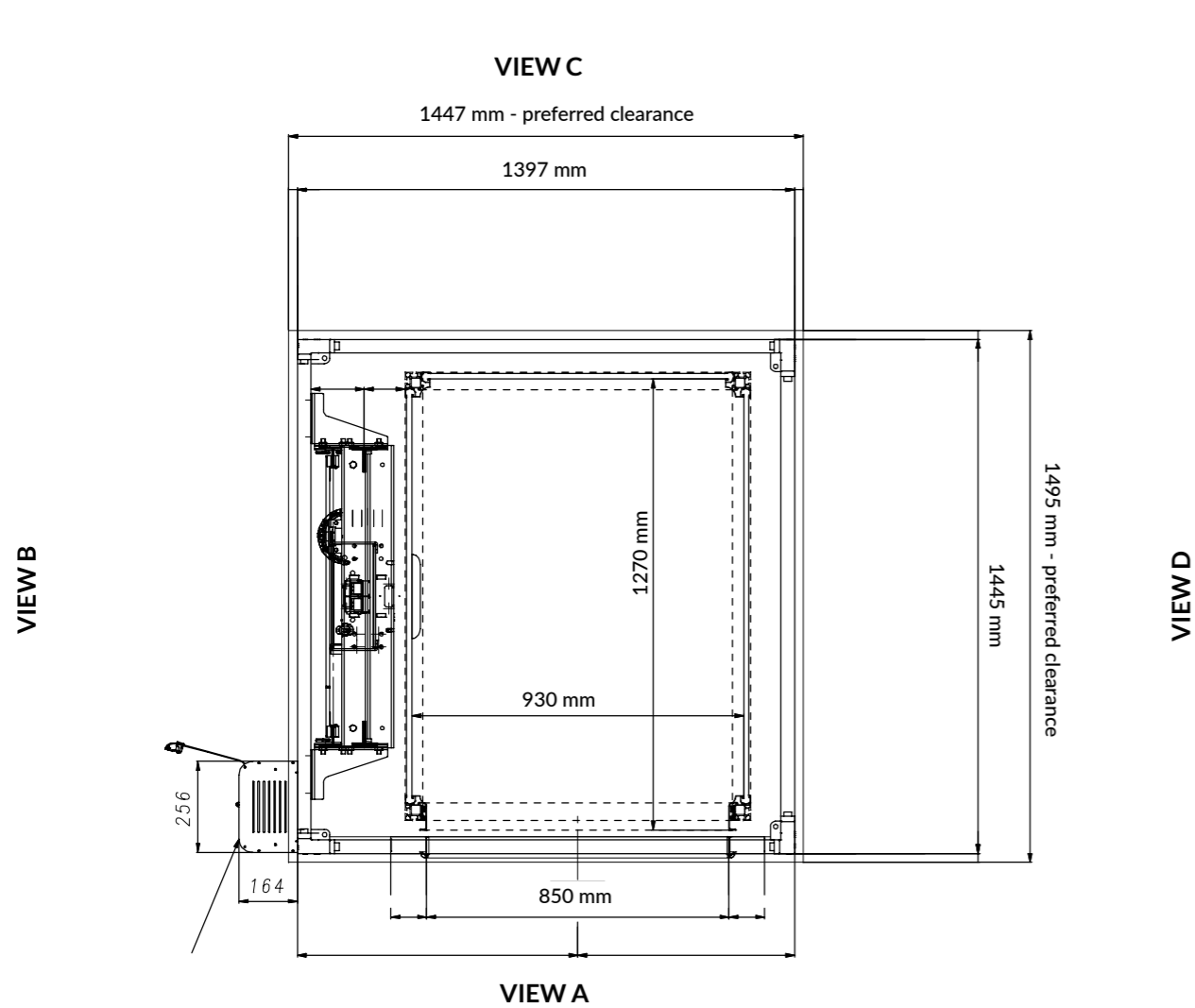
Electronics cabinet H = 1980 mm on the bottom floor
